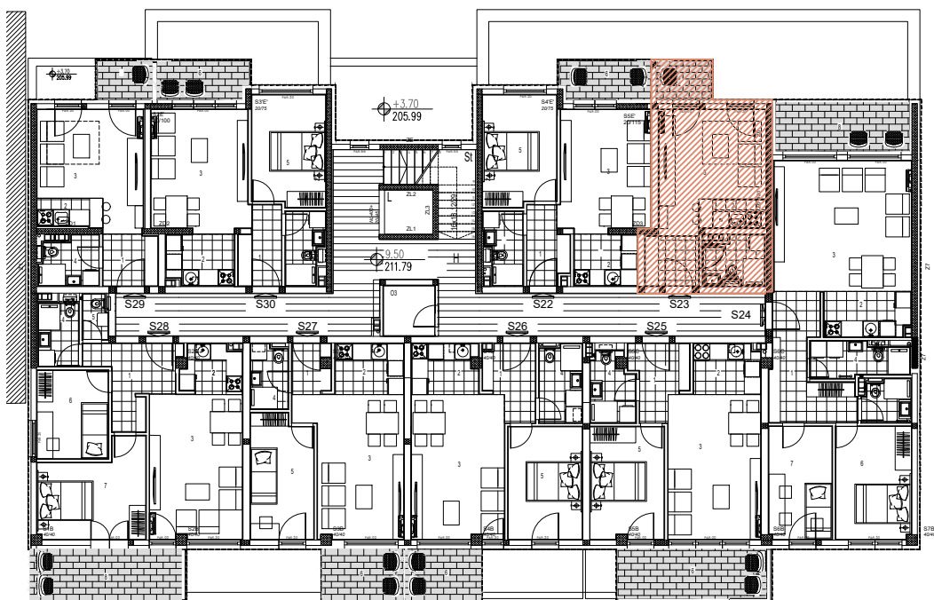
OSNOVA III.SPRATA
